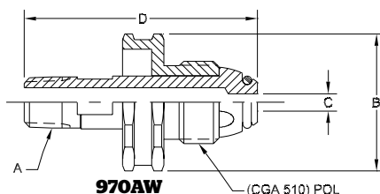
970AW 970HT Soft Nose POL w/Handwheel
