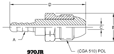
970JR Hard Nose POL w/Hose Barb Connection
