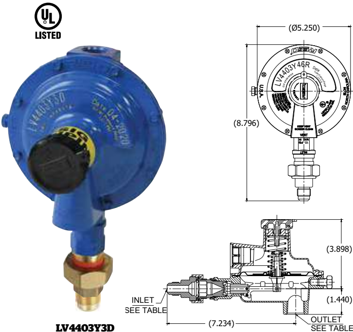
LV4403Y3D LV4403Y4D, LV4403Y46RD
