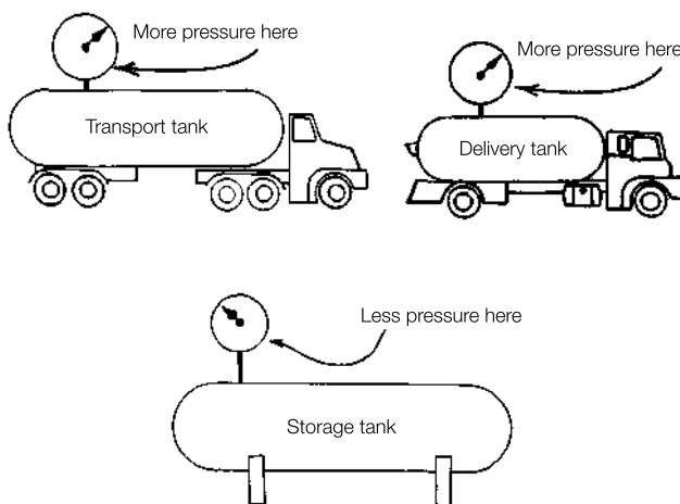
Figure 4. Unloading Conditions Affect Pressure
