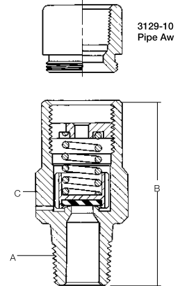
3125 Series (.161" Orifice)*** 3127 Series (.274" Orifice)**** 3129 Series (.386" Orifice)***
