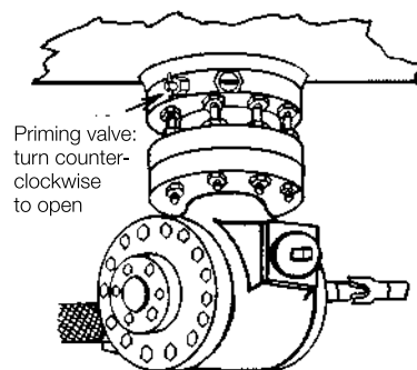
Figure 6. Priming Procedures
