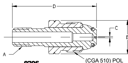
970S Soft Nose POL w/60 DMS Orifice
